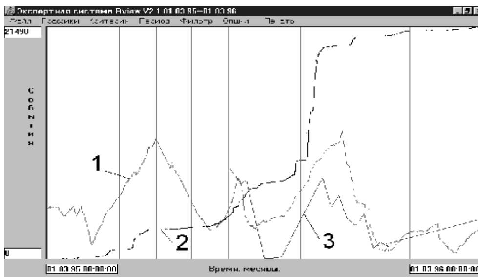
Figure 3. Trends 1 – Product level, 2 – AE activity, 3 – Product concentration in interwall space.
