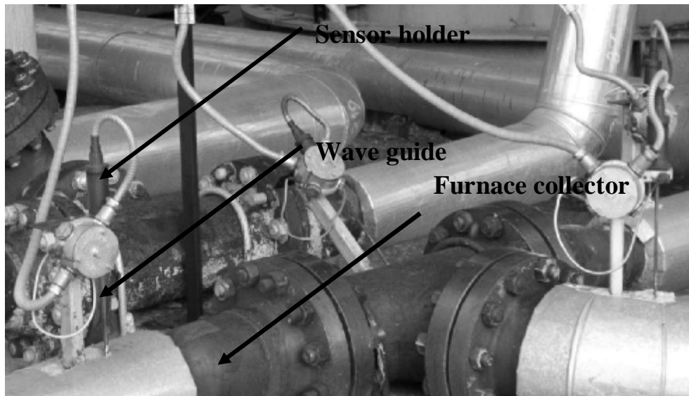
Figure 5. Sensors and wave guides
