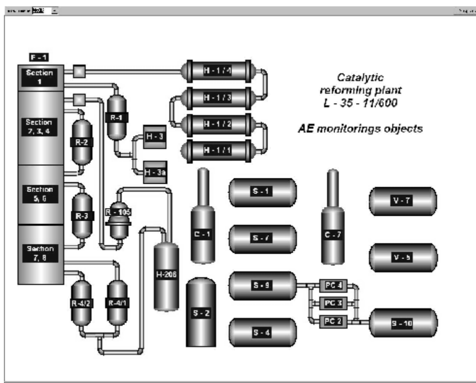
Figure 4. The schema of the controllable equipment of the reforming plant
