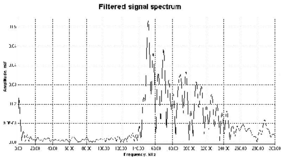
Figure 7. Noise filtering
