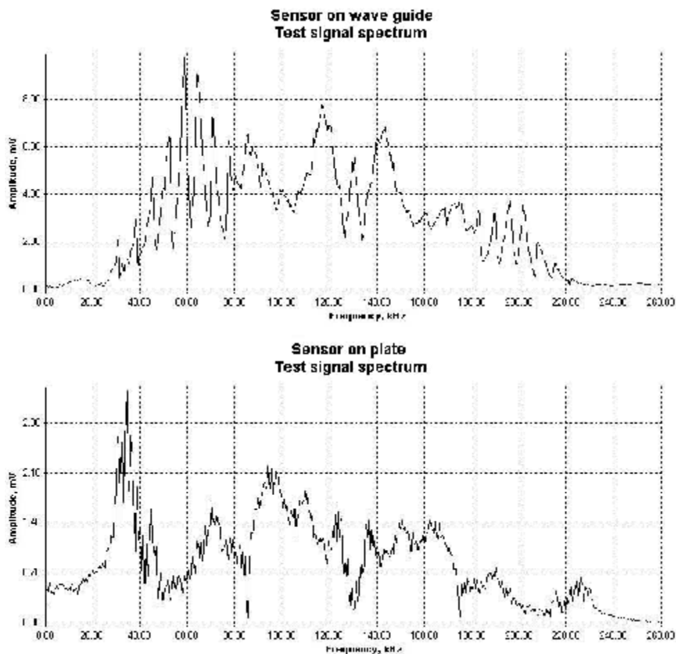
Figure 6. Signal propagation via wave guide
